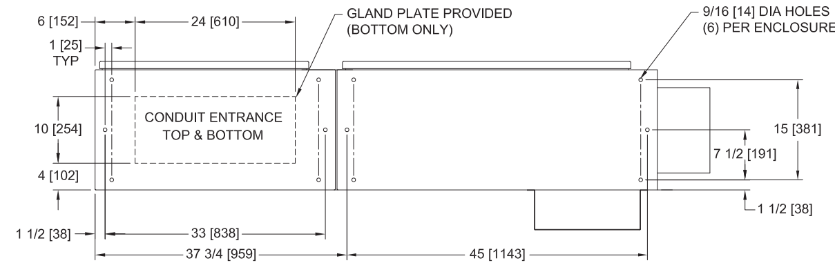
BOTTOM VIEW
